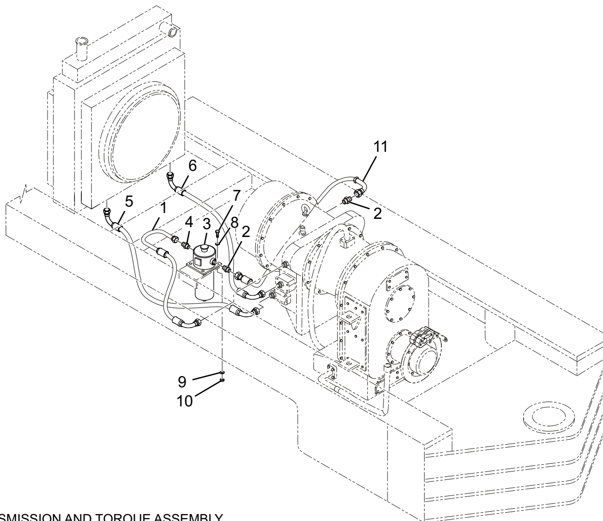
OIL CIRCUIT OF TRANSMISSION AND TORQUE ASSEMBLY
